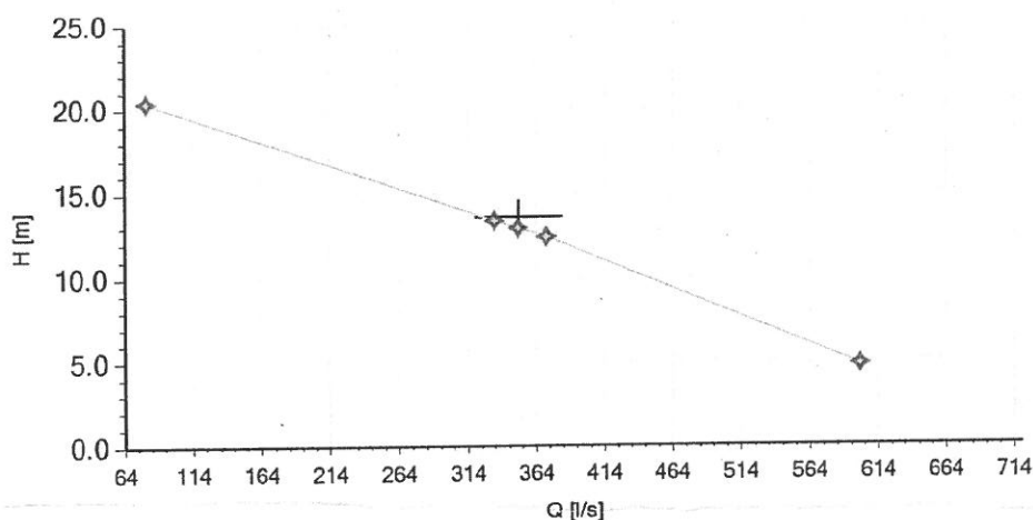
Measured values for tested pump
